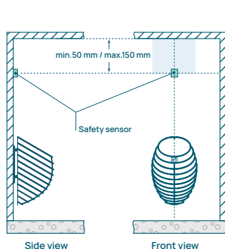
Figure 5. Installing safety sensor on the wall: wall-mounted heater
