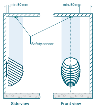
Figure 6. Installing safety sensor on the ceiling: wall-mounted heater
