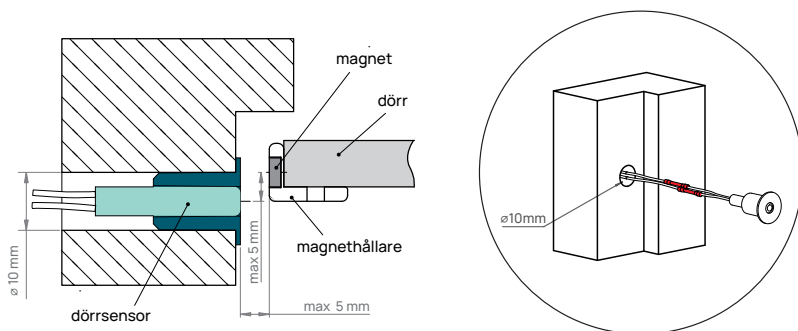
Figur 2. Dörrsensorns placering.
